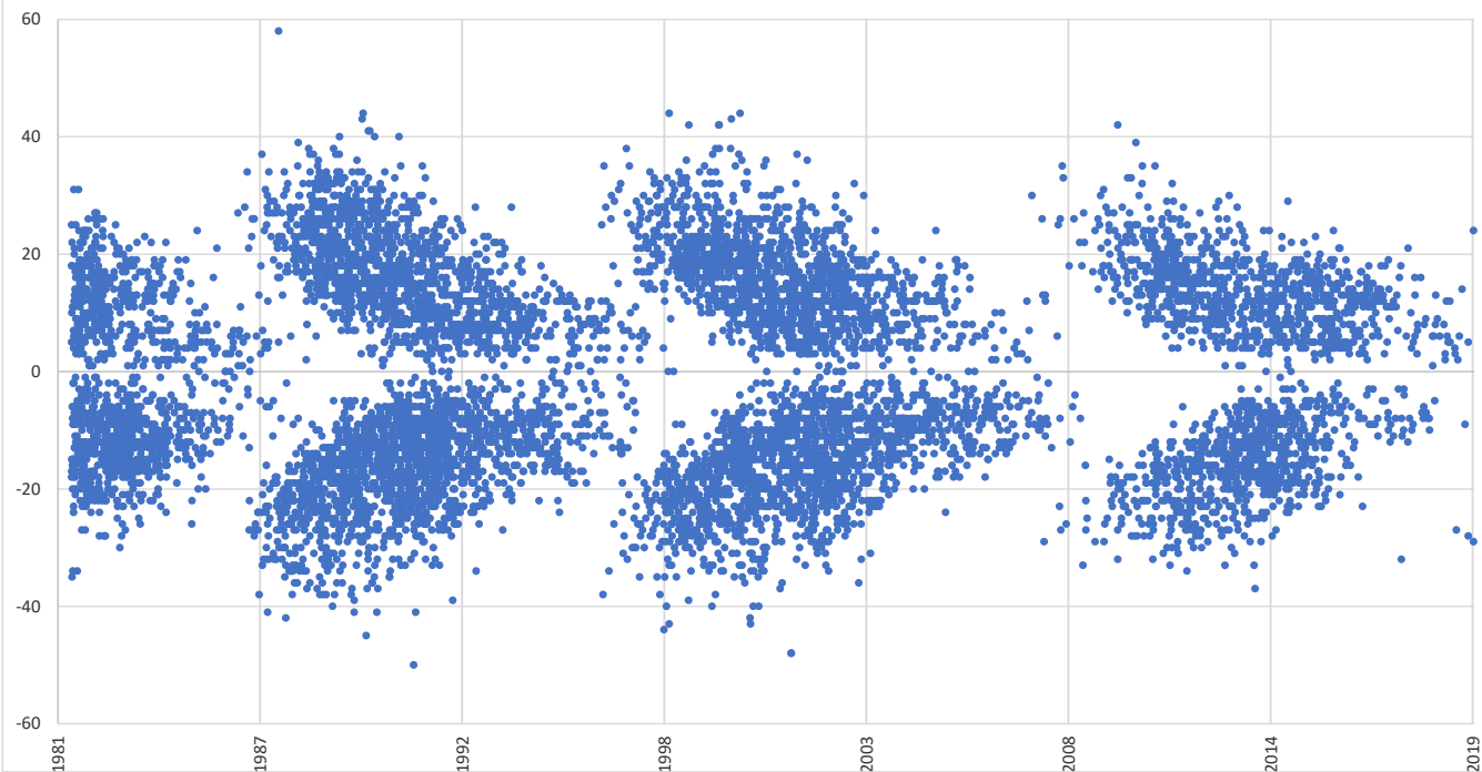
RG0/NOAA-USAF Sunspot Regions 1981-2019
