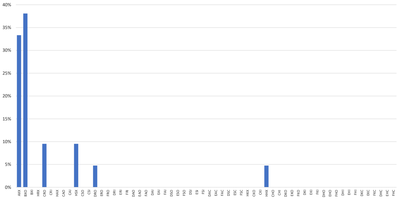
Zürich/McIntosh-classifications denoted by NOAA/USAF for the year 2019
