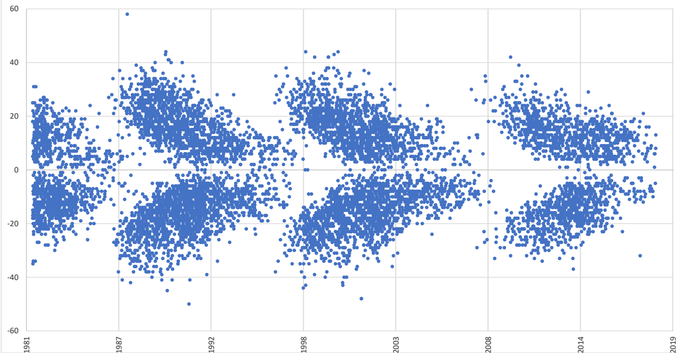
RG0/NOAA-USAF Sunspot Regions 1981-2018
