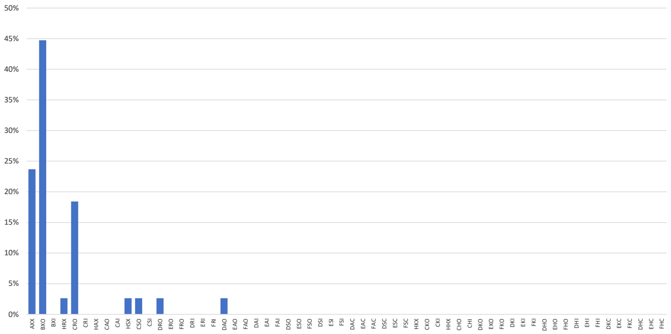
Zürich/McIntosh-classifications denoted by NOAA/USAF for the year 2018
