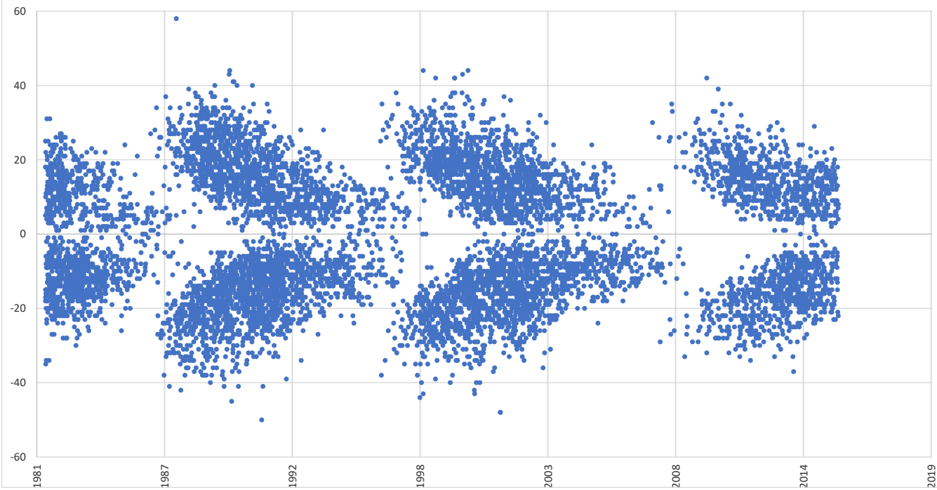
RGO/NOAA-USAF Sunspot Regions 1981-2015
