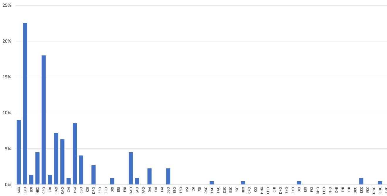
Zürich/McIntosh-classifications denoted by NOAA/USAF for the year 2015
