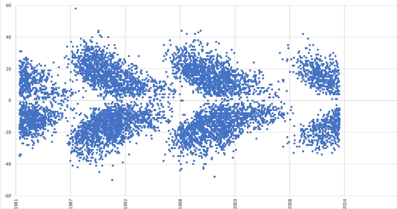
RGO/NOAA-USAF Sunspot Regions 1981-2013
