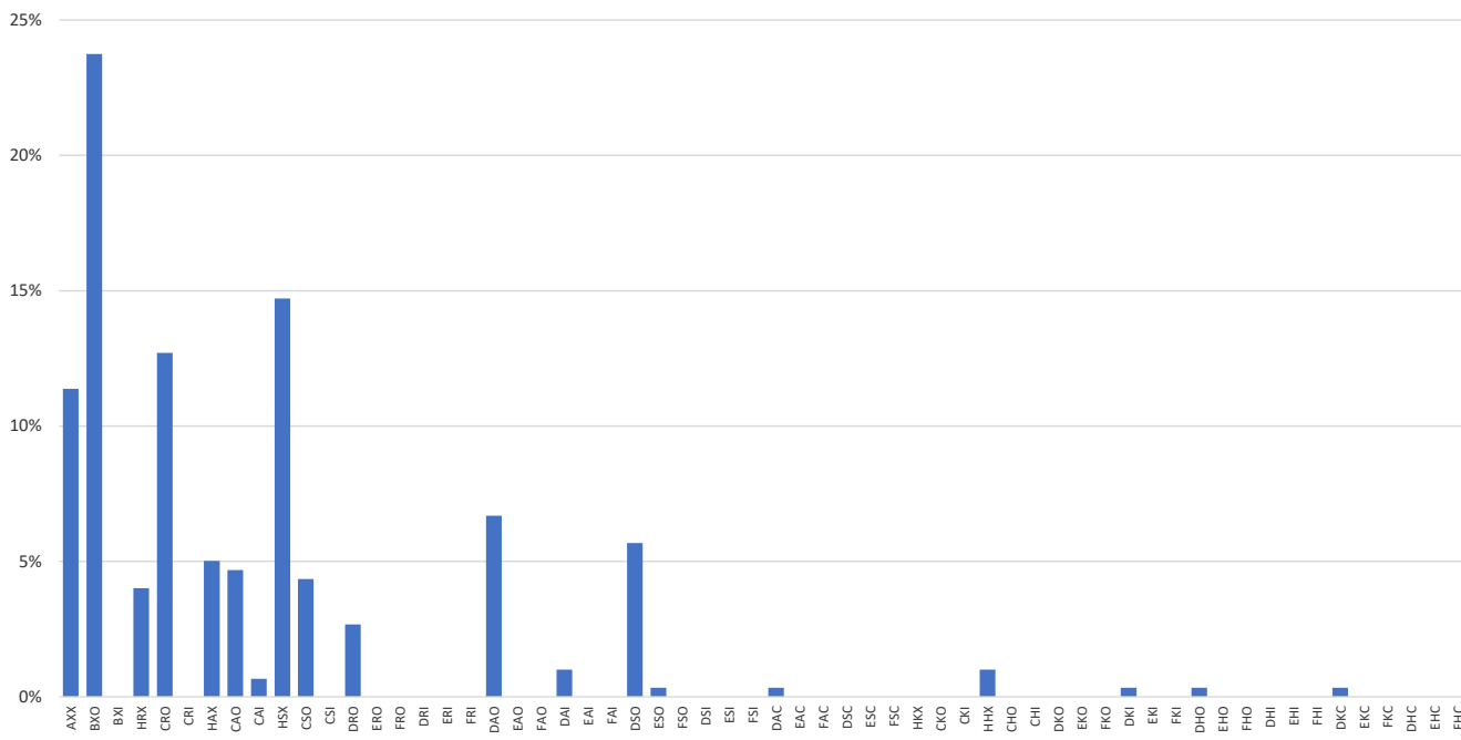
Zürich/McIntosh-classifications denoted by NOAA/USAF for the year 2013
