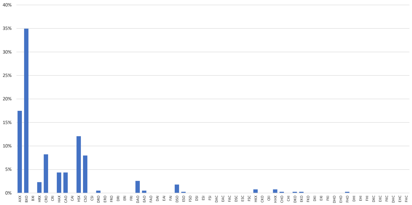
Zürich/McIntosh-classifications denoted by NOAA/USAF for the year 1999
