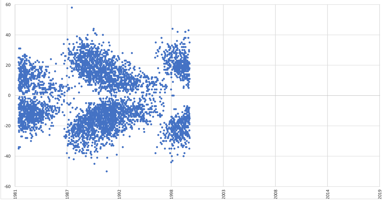
RGO/NOAA-USAF Sunspot Regions 1981-1999
