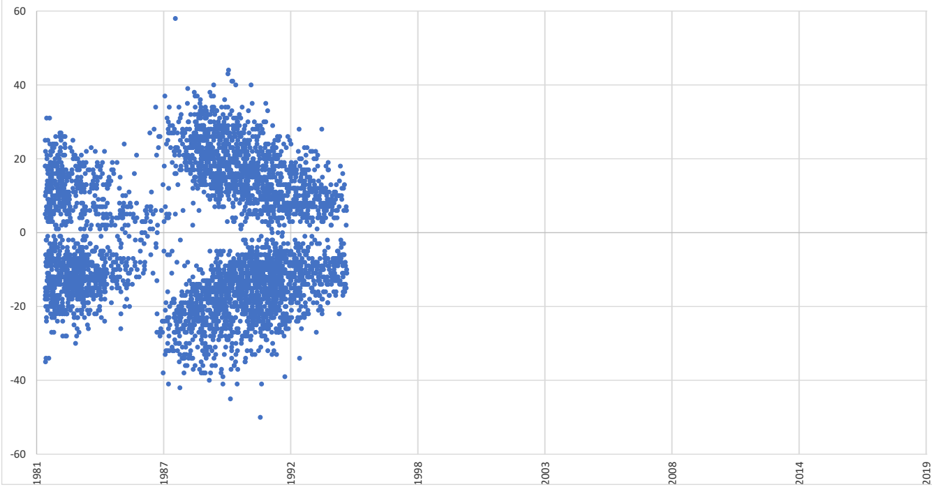
RGO/NOAA-USAF Sunspot Regions 1981-1994
