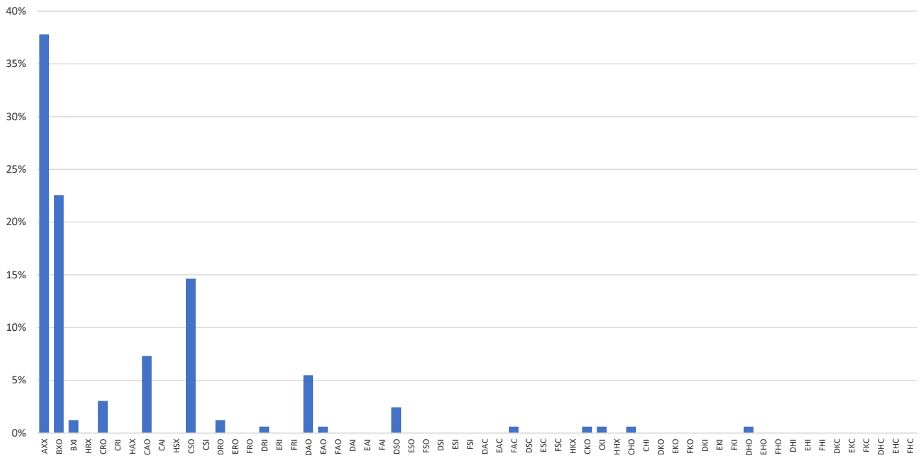
Zürich/McIntosh-classifications denoted by NOAA/USAF for the year 1994
