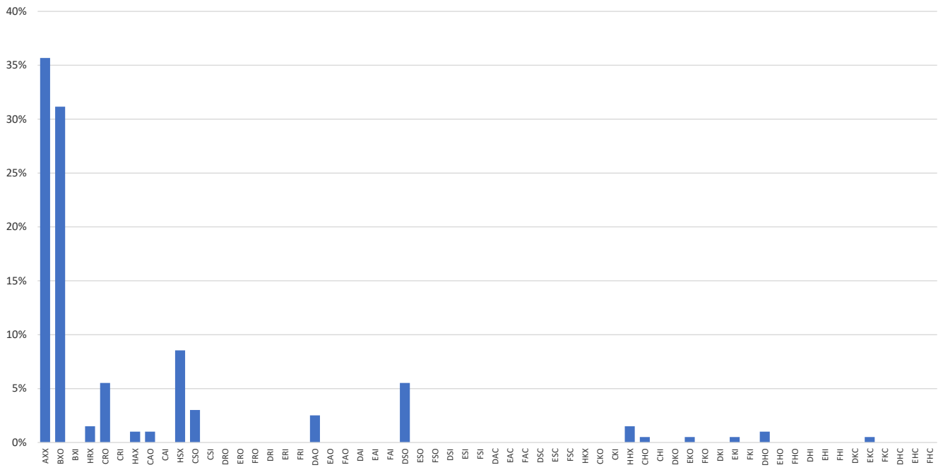
Zürich/McIntosh-classifications denoted by NOAA/USAF for the year 1984
