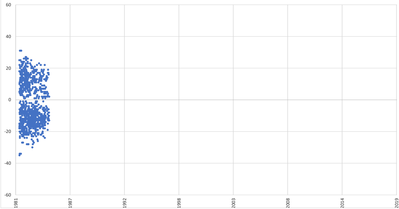
RGO/NOAA-USAF Sunspot Regions 1981-1984
