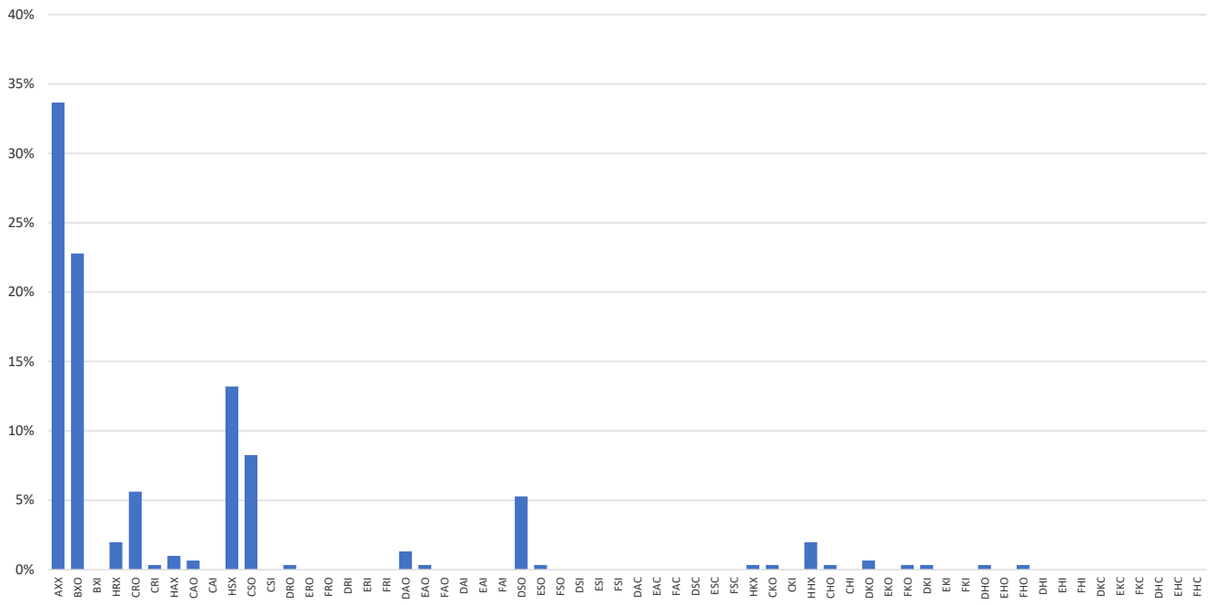
Zürich/McIntosh-classifications denoted by NOAA/USAF for the year 1983
