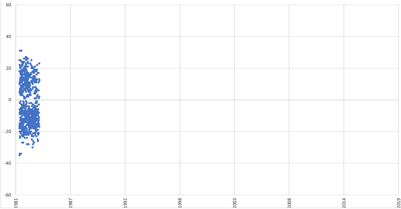
RGO/NOAA-USAF Sunspot Regions 1981-1983
